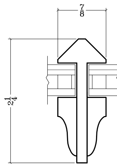
1 MUNTIN DETAIL S3 FULL SCALE
